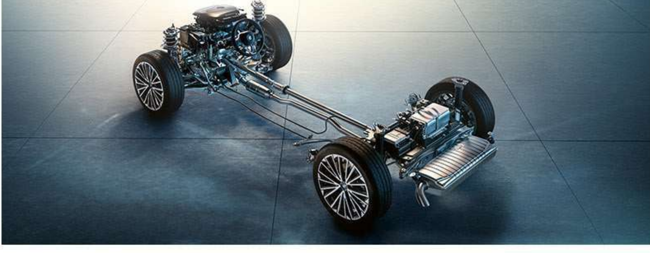
M Adaptive Suspension: Dynamic Damper Control, frequency-selective damping elements: mechanical, self-regulating system with regulation depending on road condition and driving style, also includes M Sport steering which allows for more direct steering feedback with lower steering effort.
